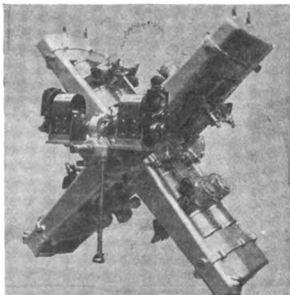
Cross-Shaped Gobron.
